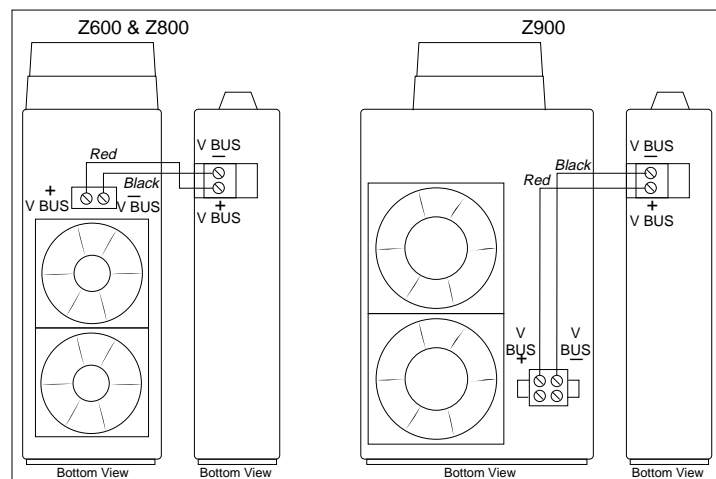
Shunt Regulator Installation
