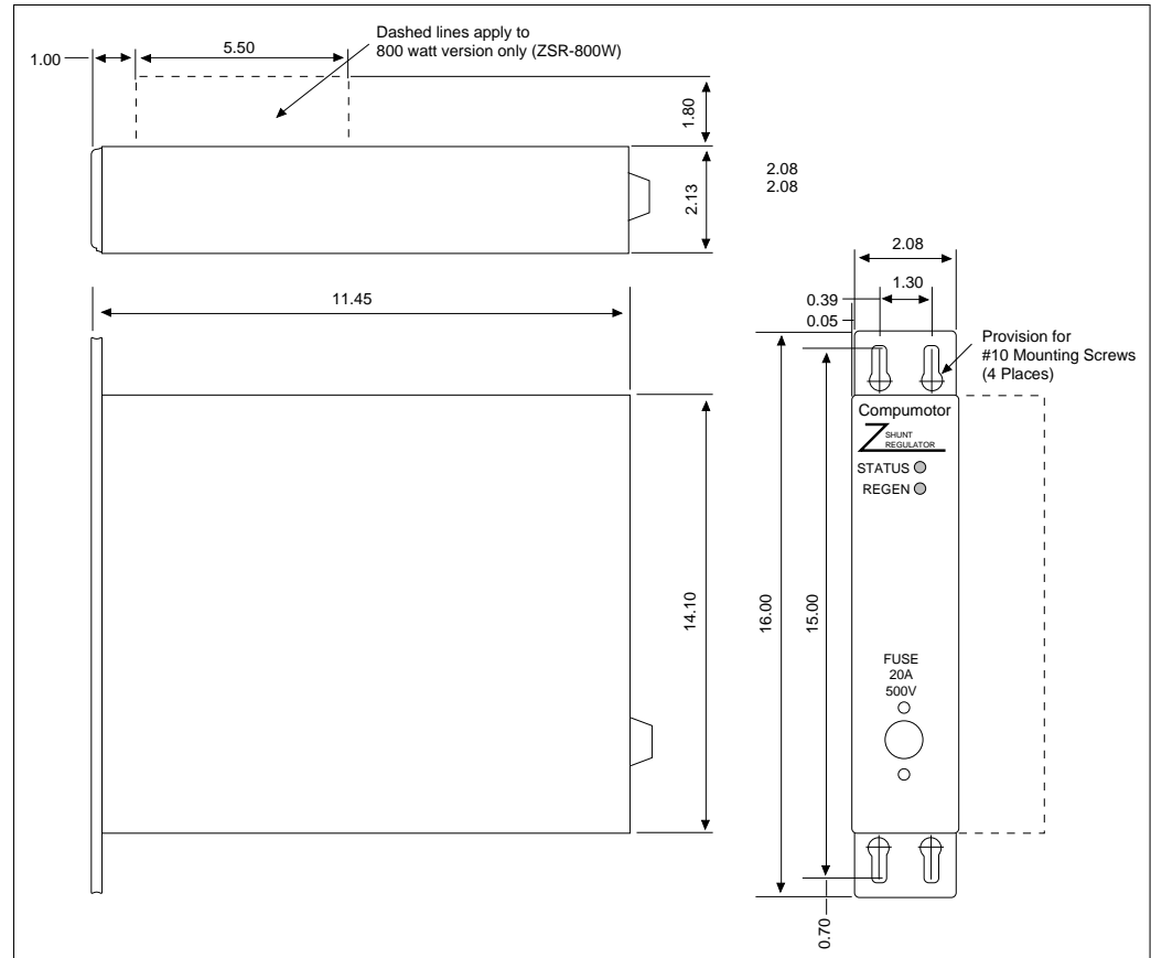
Z Series Shunt Regulator Dimensions
