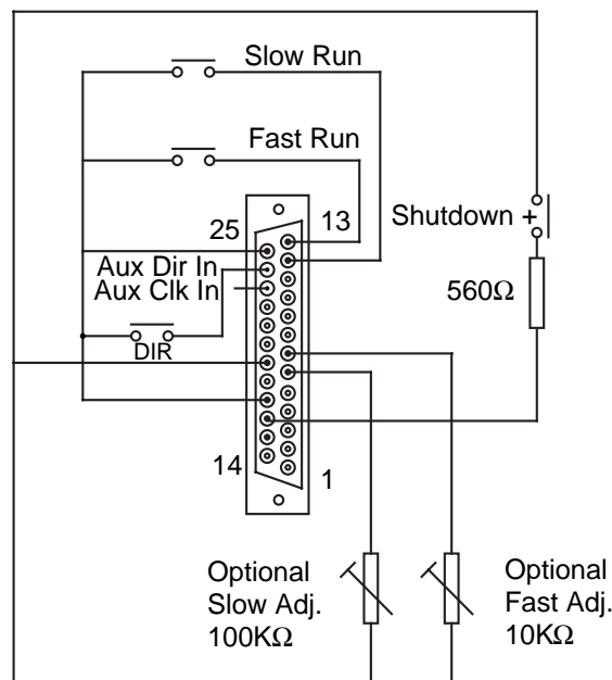
Figure 3-10. Signal Connections
