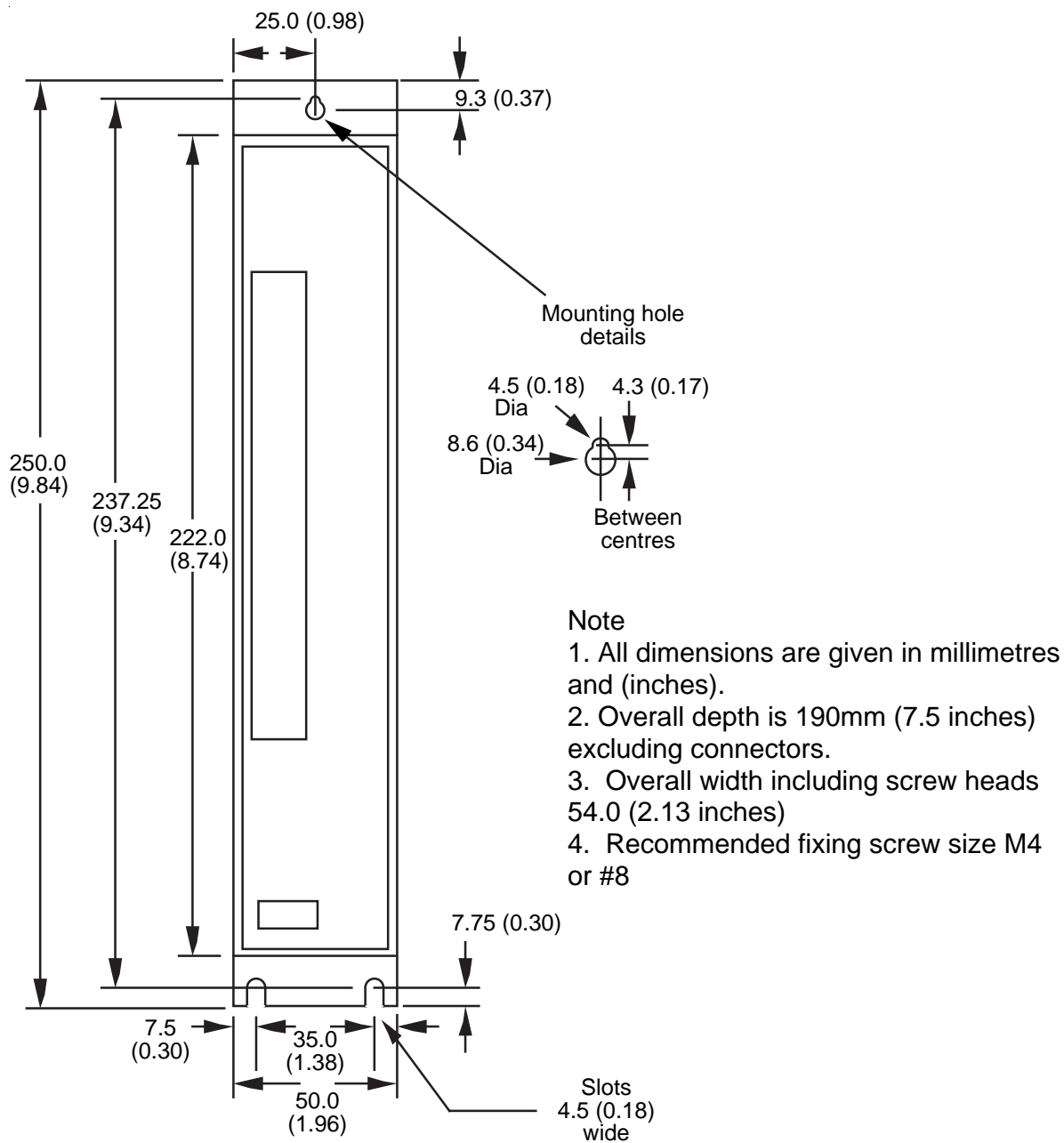
Figure 3-12 Drive Mounting Hole Locations
