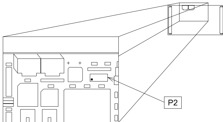
Figure 1.15 Factory test connector
