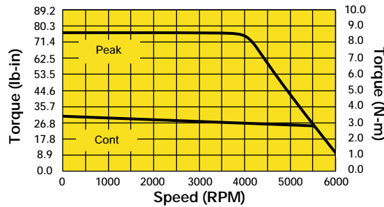
HDY115A6-88S w/COMPAX200M (460VAC)
