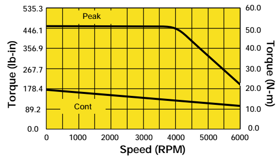
HBMR190J6-260S w/COMPAX1500M (460VAC)
