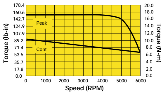
HBMR190E6-88S w/COMPAX1500M (460VAC)
