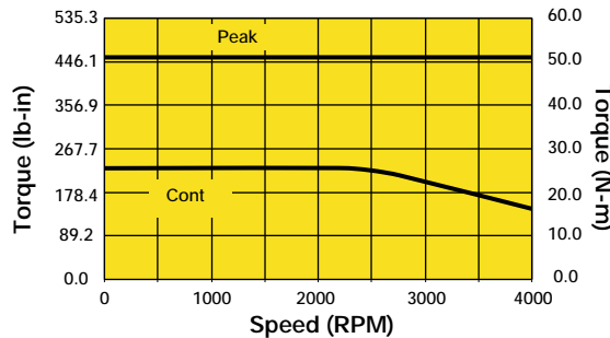
HBMR190E6-88S w/COMPAX1500M (460VAC)
