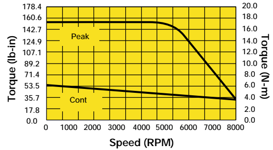
HDY142G6-88S w/COMPAX1500M (460VAC)
