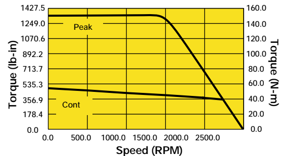
HBMR190J6-260S w/COMPAX1500M (460VAC)
