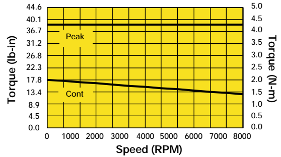
HDY115C6-88S w/COMPAX500M (460VAC)
