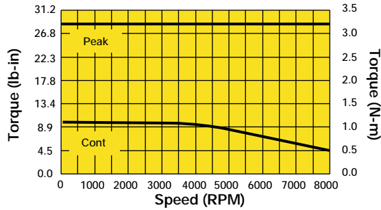
HDY70C4-44S w/COMPAX200M (460VAC)
