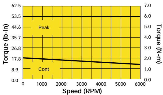
HDY115C6-88S w/COMPAX8500S (460VAC)
