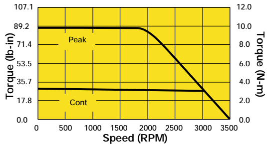
HDY115A6-88S w/COMPAX2500 (230VAC)
