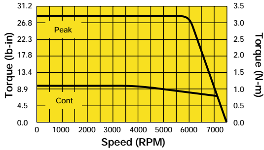
HDY115A6-88S w/COMPAX2500 (230VAC)
