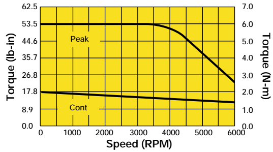
HDY70C4-44S w/COMPAX4500S (460VAC)
