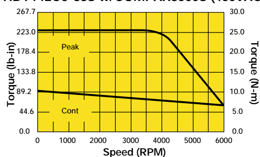
HDY142C6-88S w/COMPAX8500S (460VAC)
