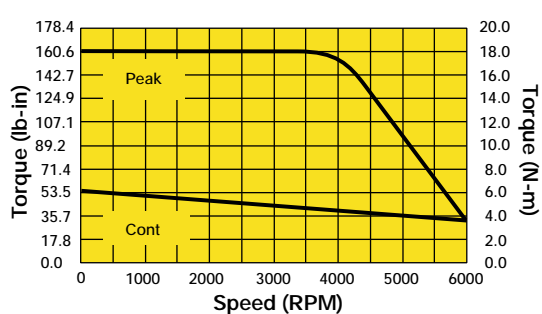
HDY115C6-88S w/COMPAX8500S (460VAC)
